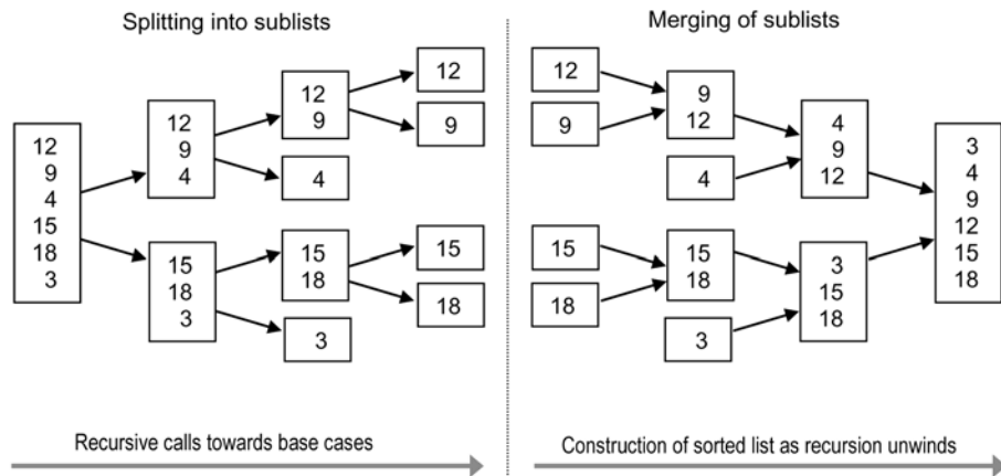
FIGURE 11-15 Recursive Problem-Solving Example (MergeSort)
