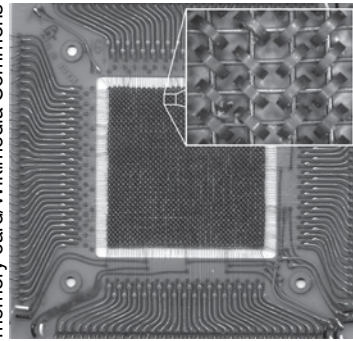
FIGURE 12-27 One Plane of Magnetic Core Memory
